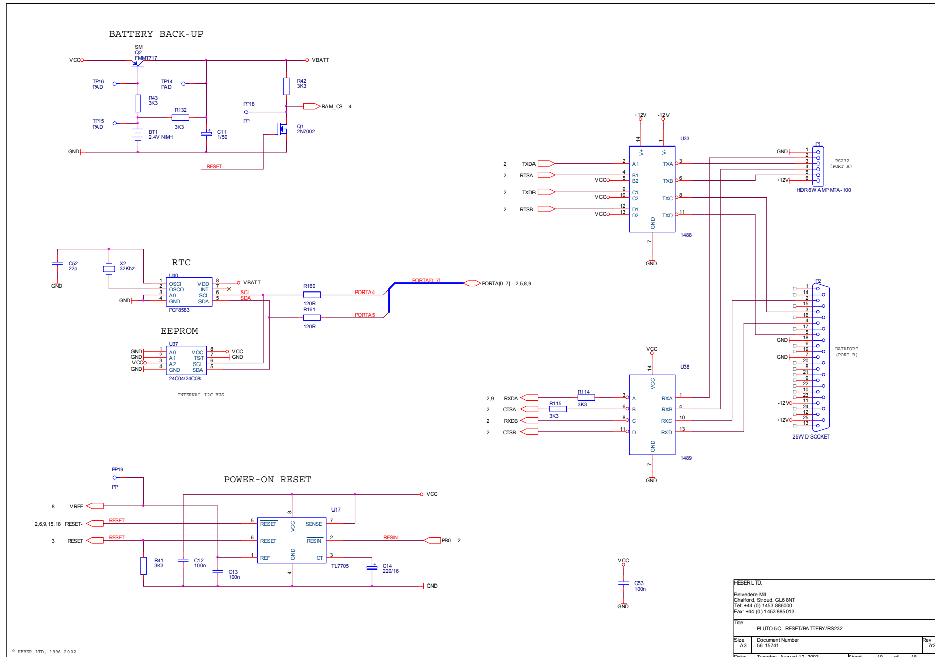
Figure 10 - Schematic Sheet 10 - Reset/Battery/RS232 Channels A &amp; B
