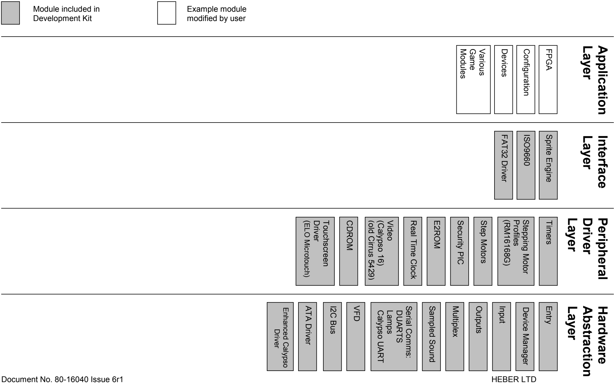
Figure 1 – Pluto 5 Software Structure
